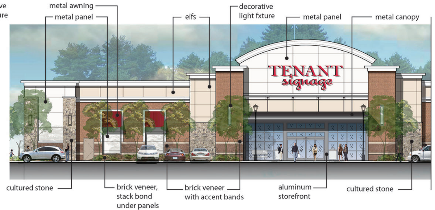
Partial Front Elevation at Building A-D
