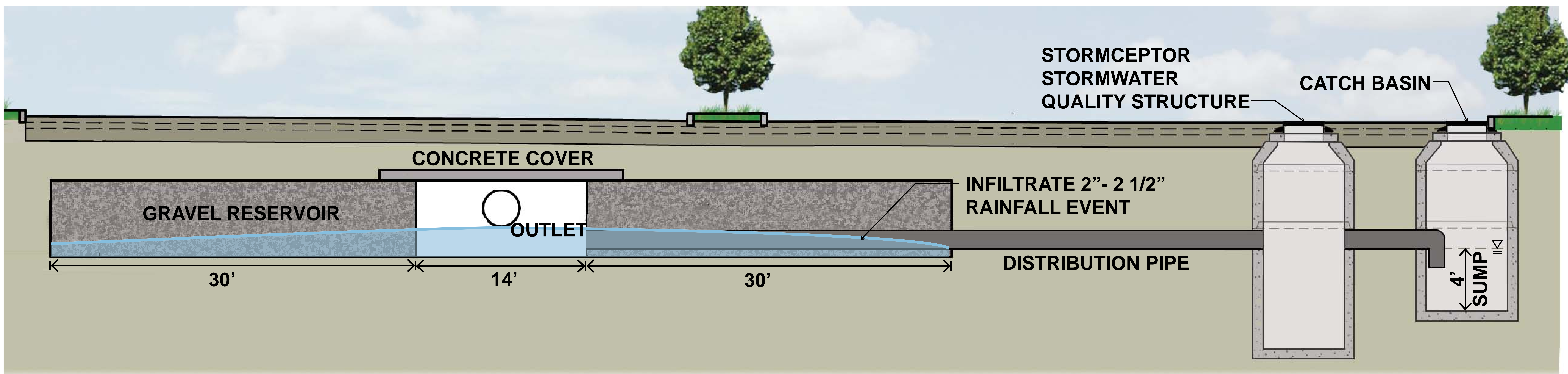
TYPICAL INFILTRATION BASIN TREATMENT TRAIN
