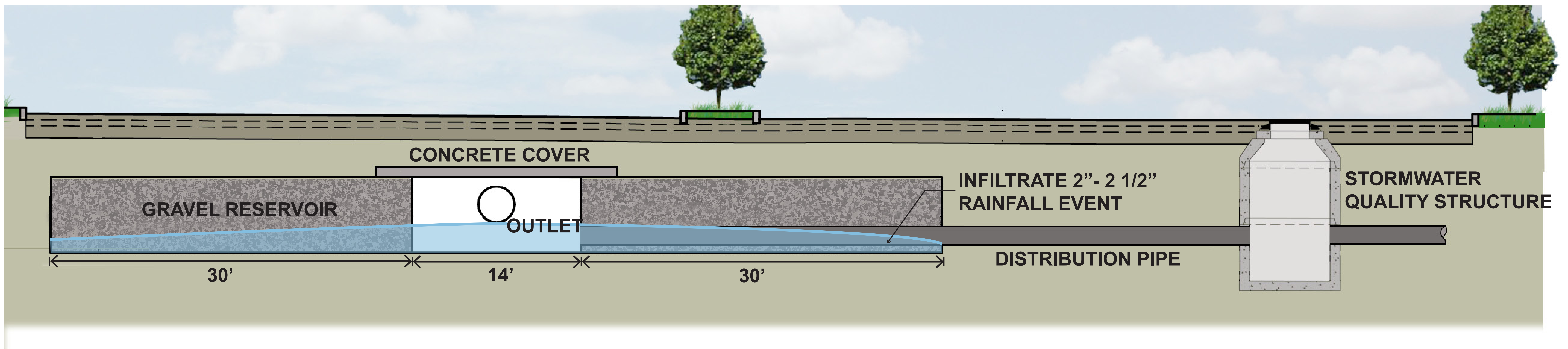
TYPICAL INFILTRATION BASIN CROSS SECTION
