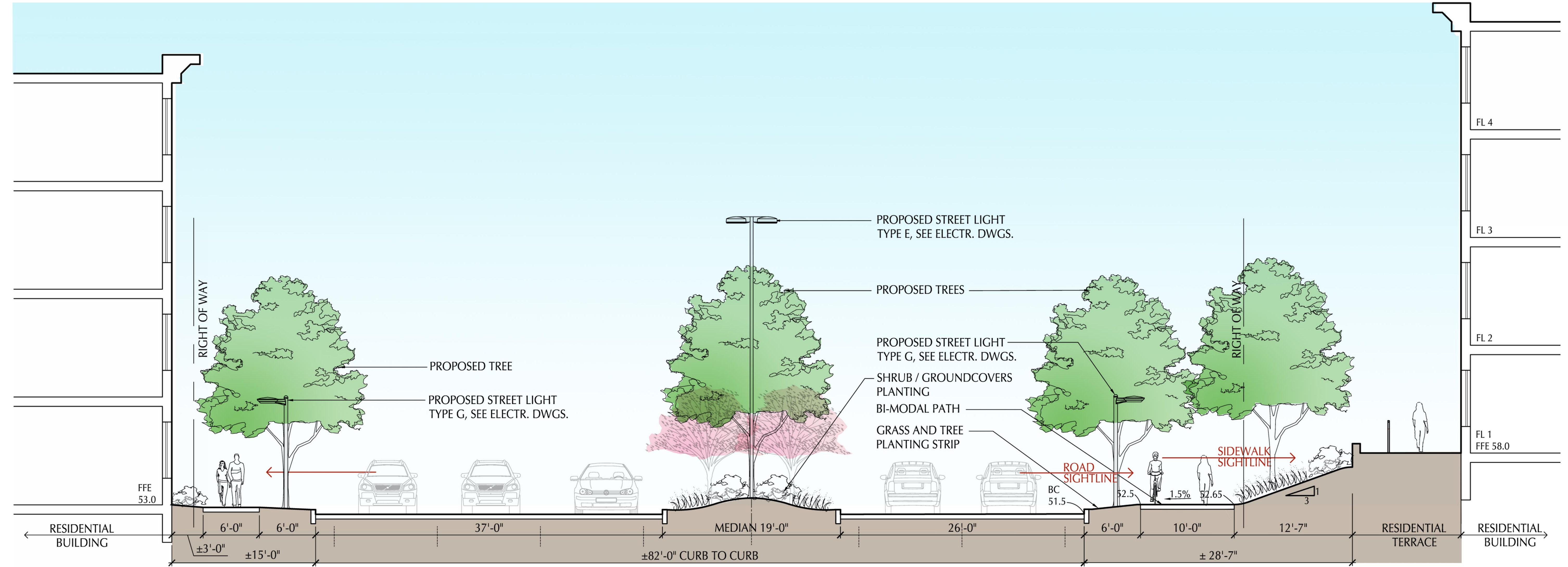
1 UNIVERSITY AVENUE SECTION A-A SCALE: 3/16" = 1'-0"
