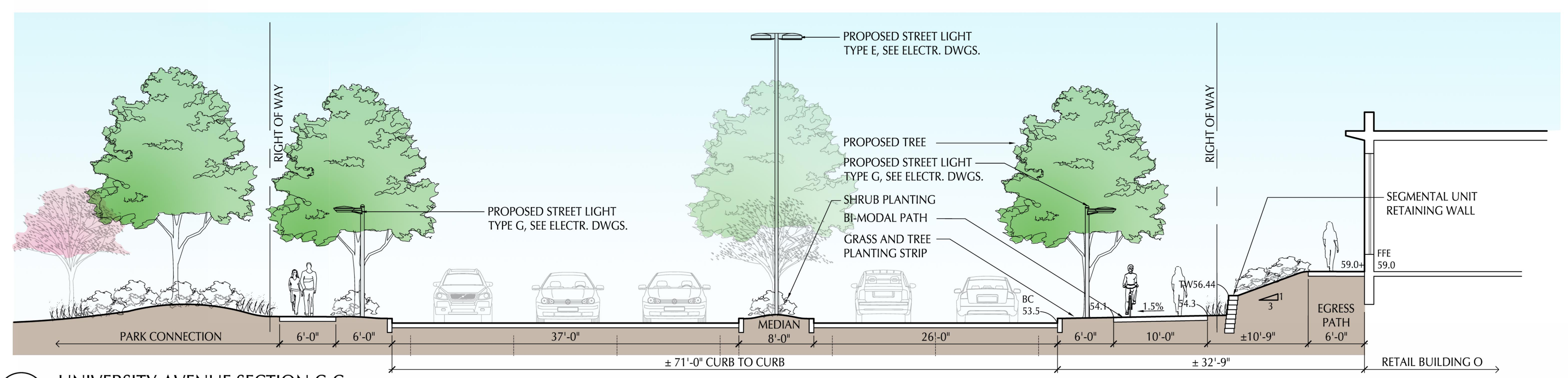
3 UNIVERSITY AVENUE SECTION C-C SCALE: 3/16" = 1'-0"
