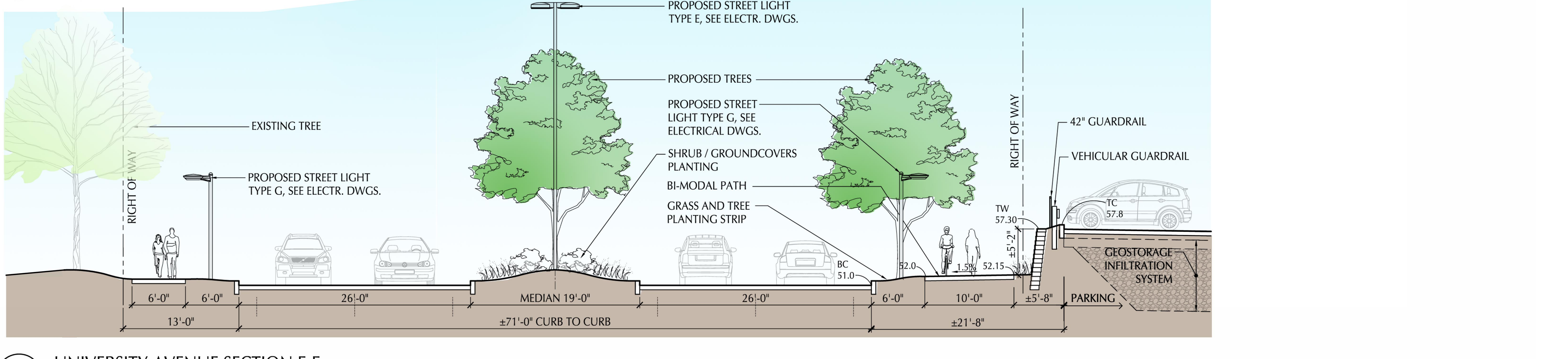
6 UNIVERSITY AVENUE SECTION F-F SCALE: 3/16" = 1'-0"
