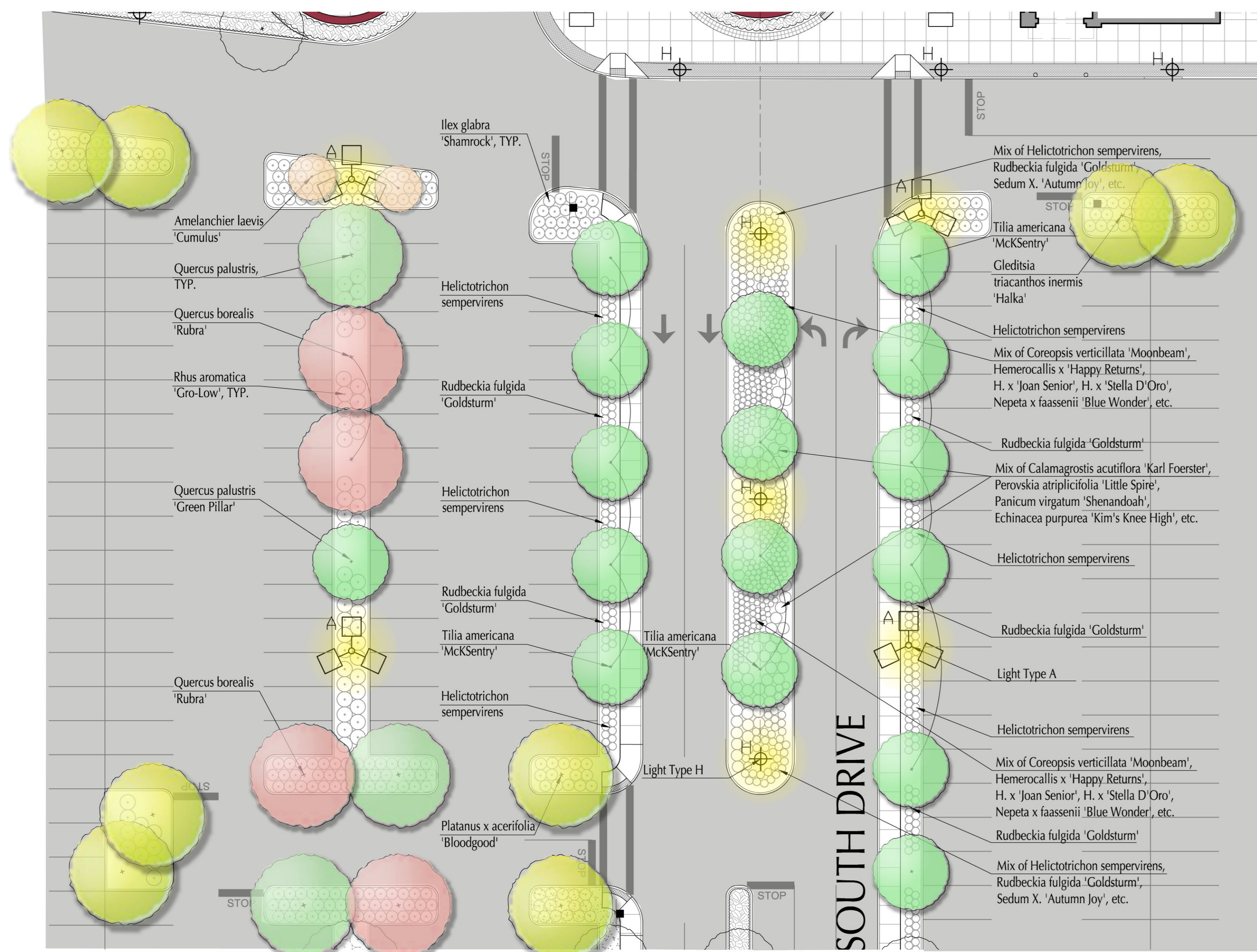
1 PLANTING PLAN ENLARGEMENT AT RETAIL PARKING LOT SCALE: 1" = 20'-0"
