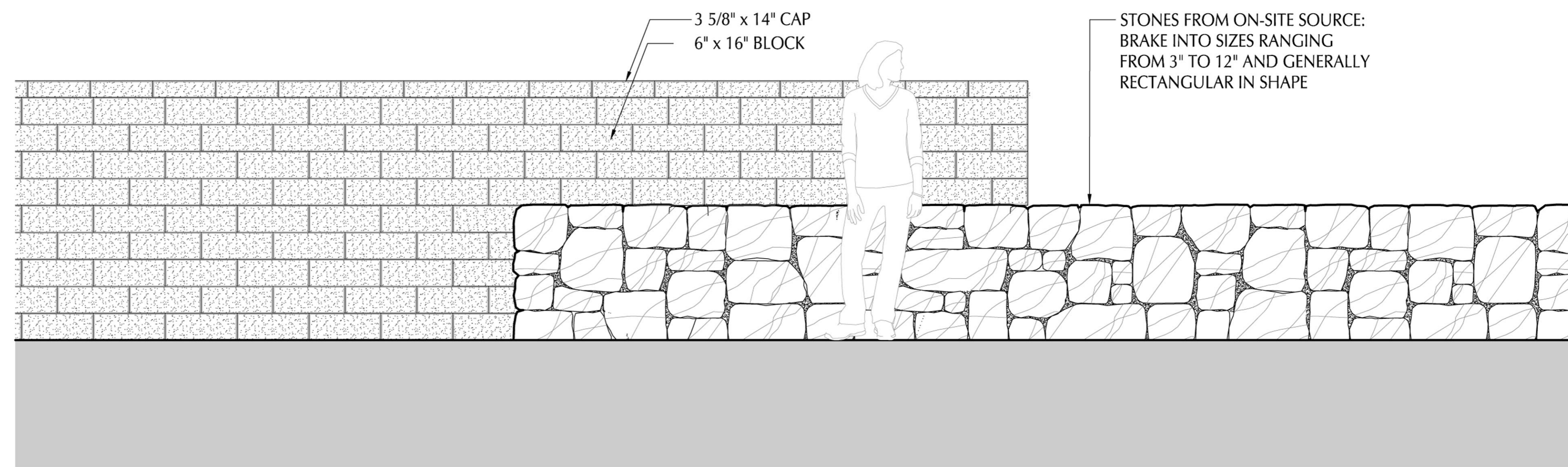
3 CONCRETE UNIT AND SALVAGED STONE WALL TYPICAL ELEVATIONS SCALE: 3/8" = 1'-0"
