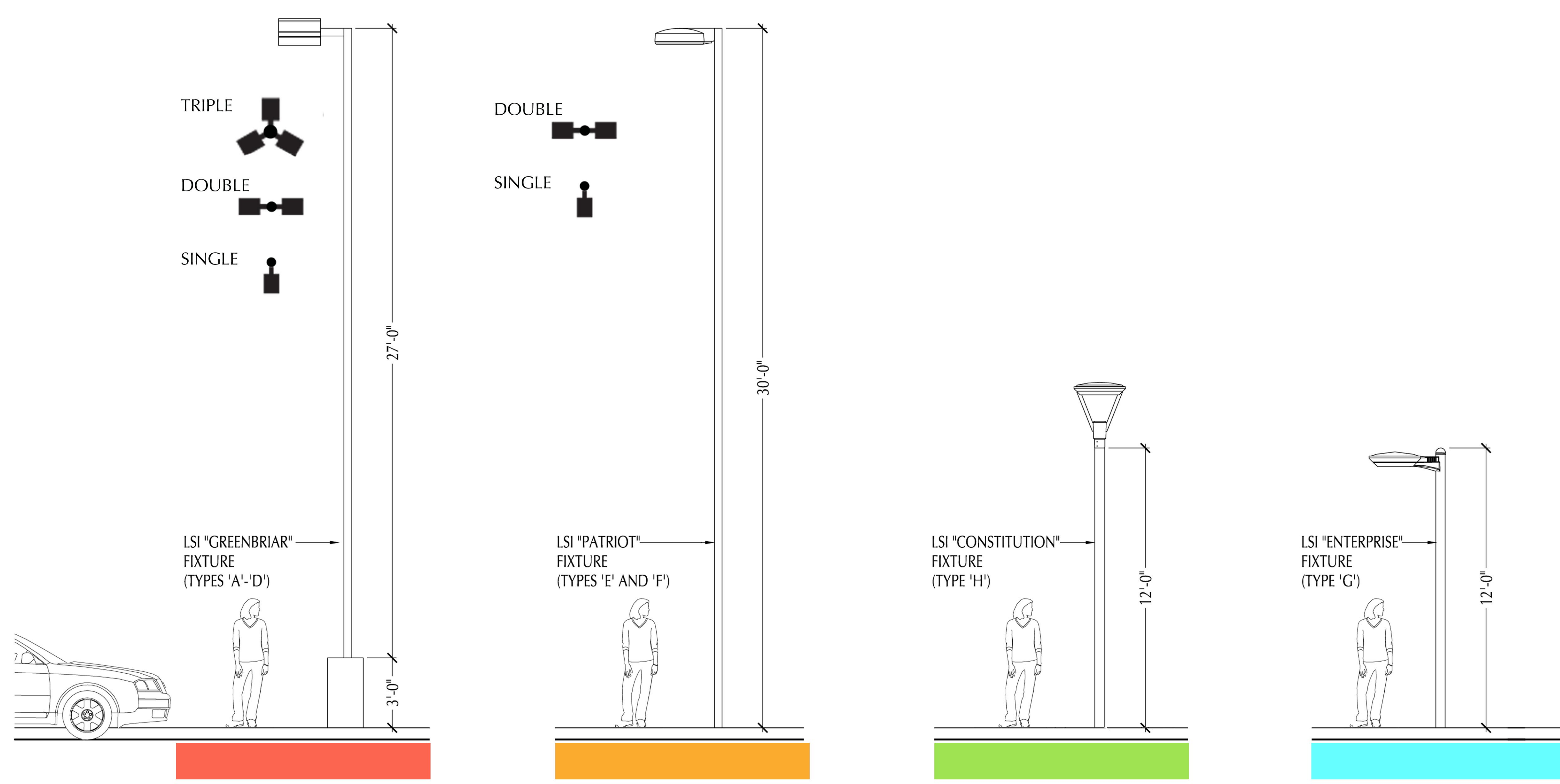
LIGHTING FIXTURE COMPARISON SCALE: 3/8" = 1'-0"
