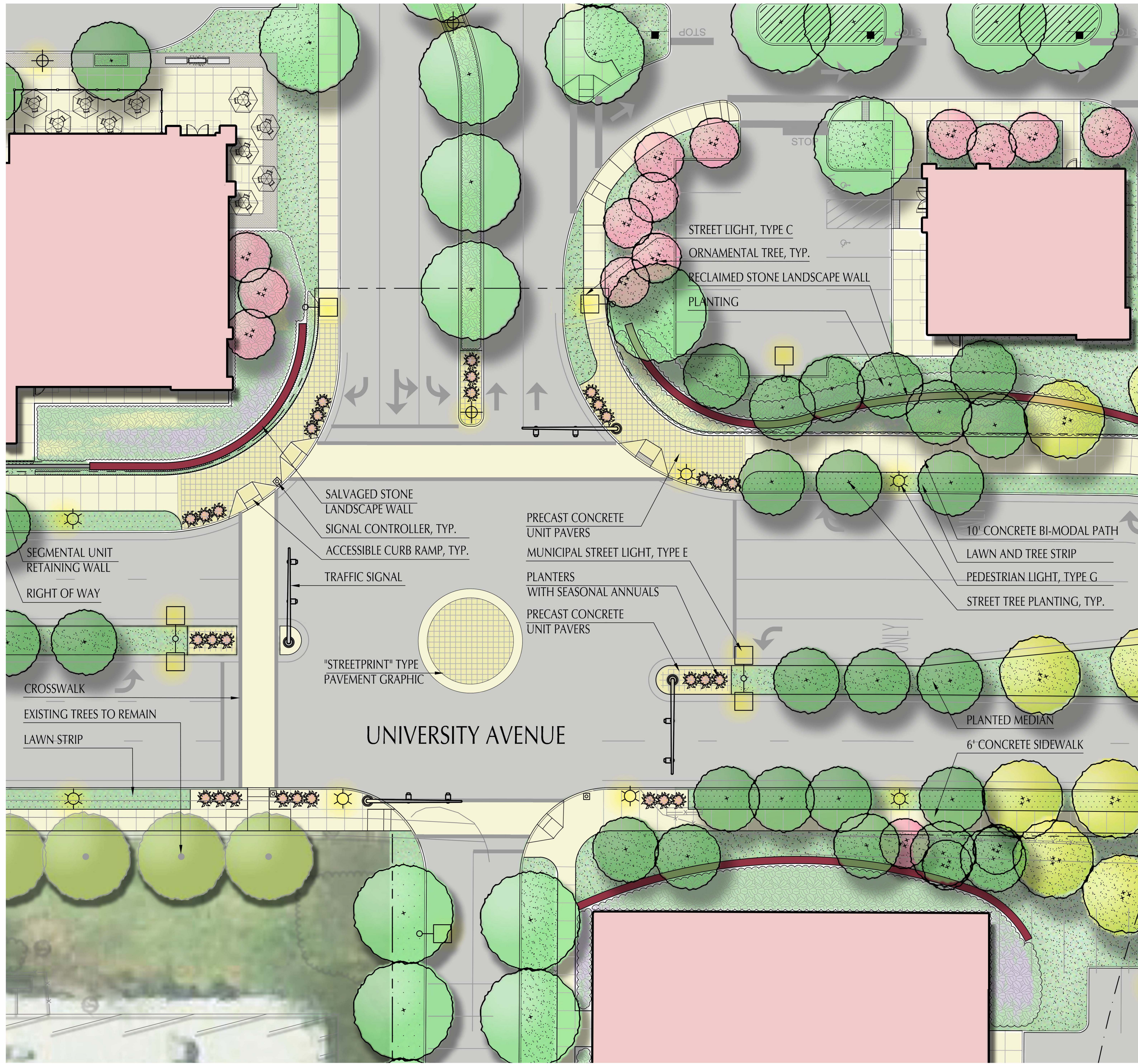
INTERSECTION 2 PLAN ENLARGEMENT SCALE: 1"=10'-0"
