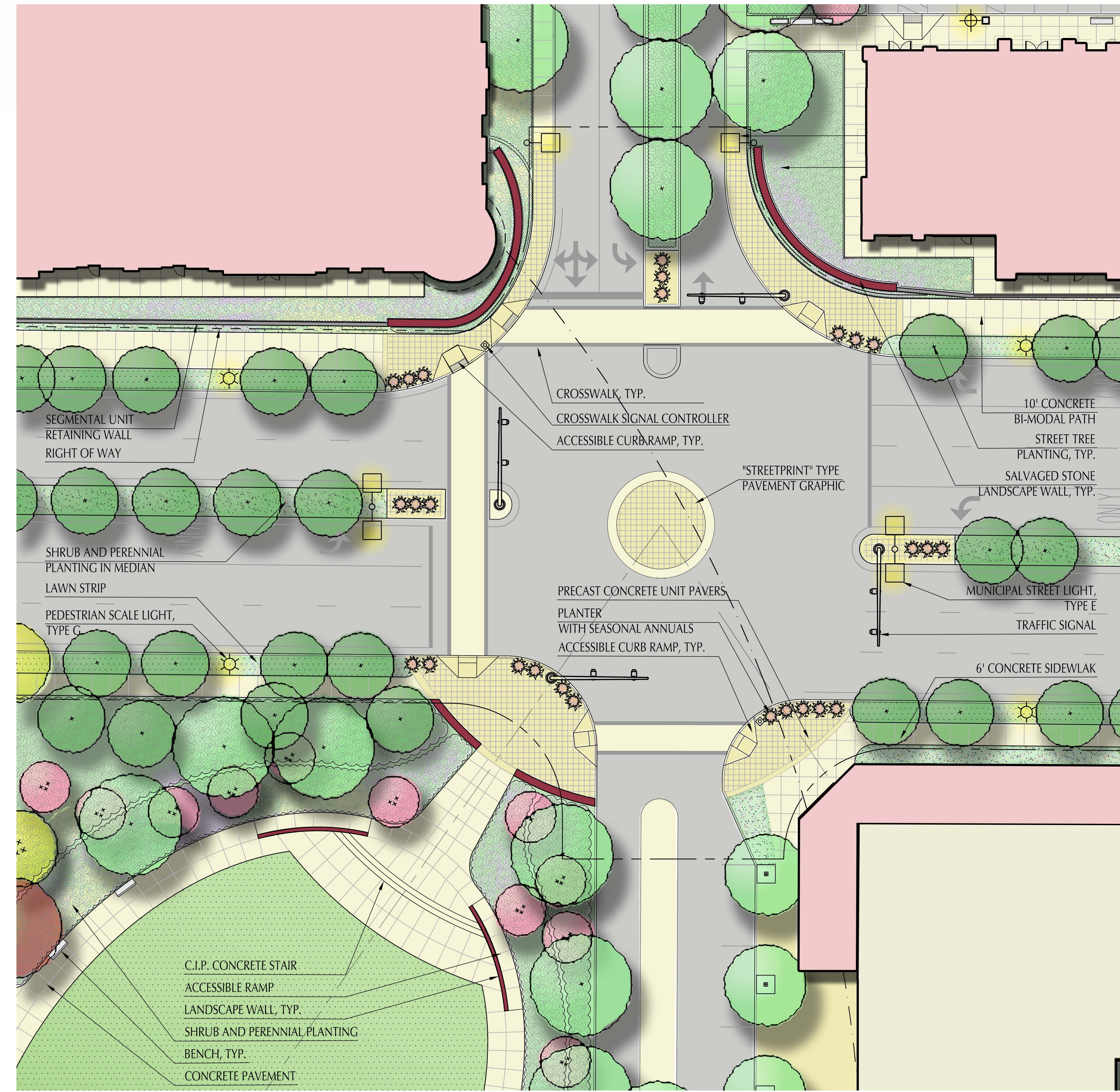
INTERSECTION 1 PLAN ENLARGEMENT SCALE: 1"=10'-0"
