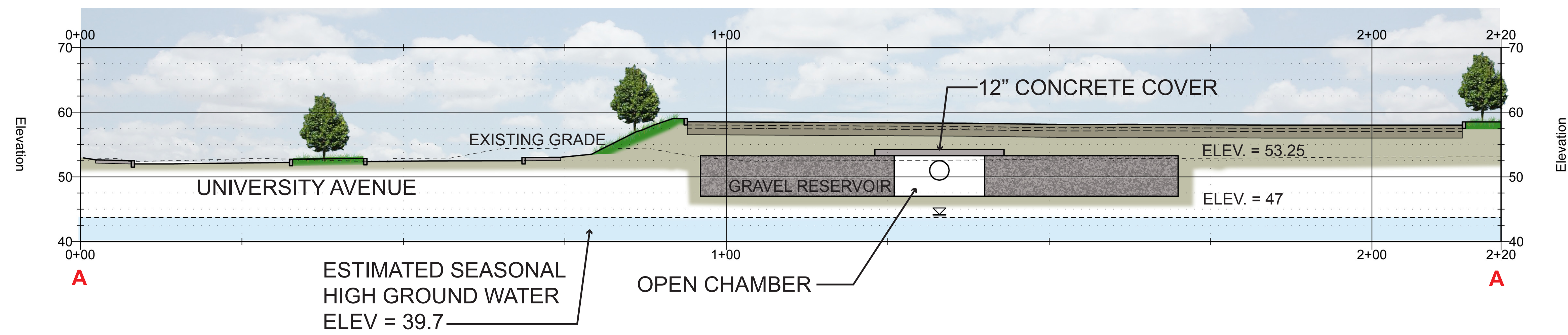
INFILTRATION BASIN CROSS SECTION A-A
