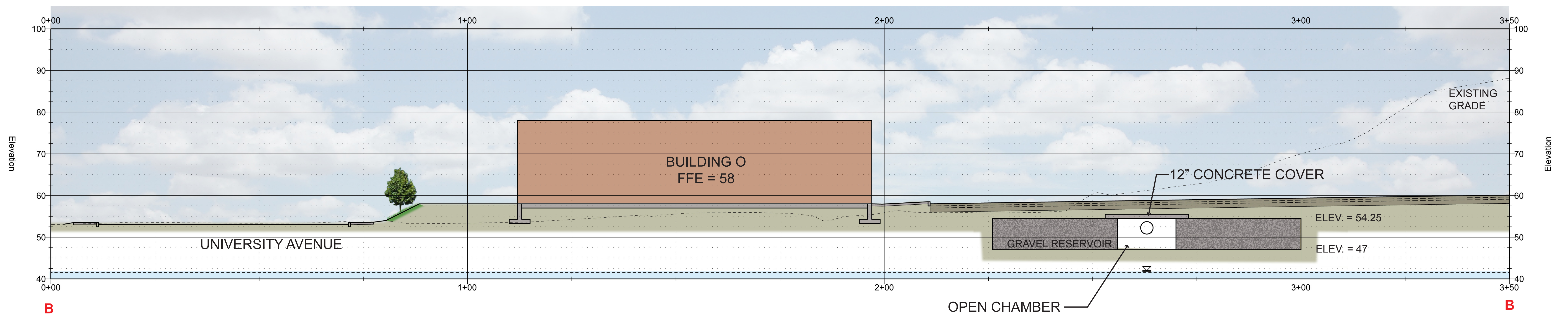
INFILTRATION BASIN CROSS SECTION B-B
