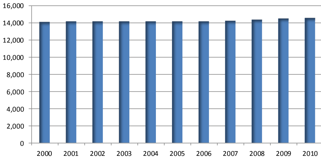
Figure 39: Population History
