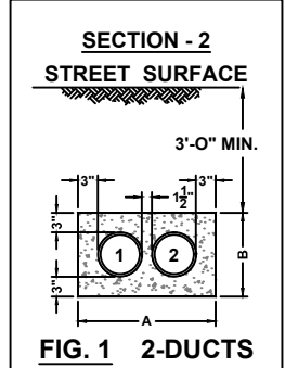
FIG. 1 2-DUCTS
